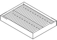
IN/L140/S IN/L140/S/M 153 x 210 x 28
